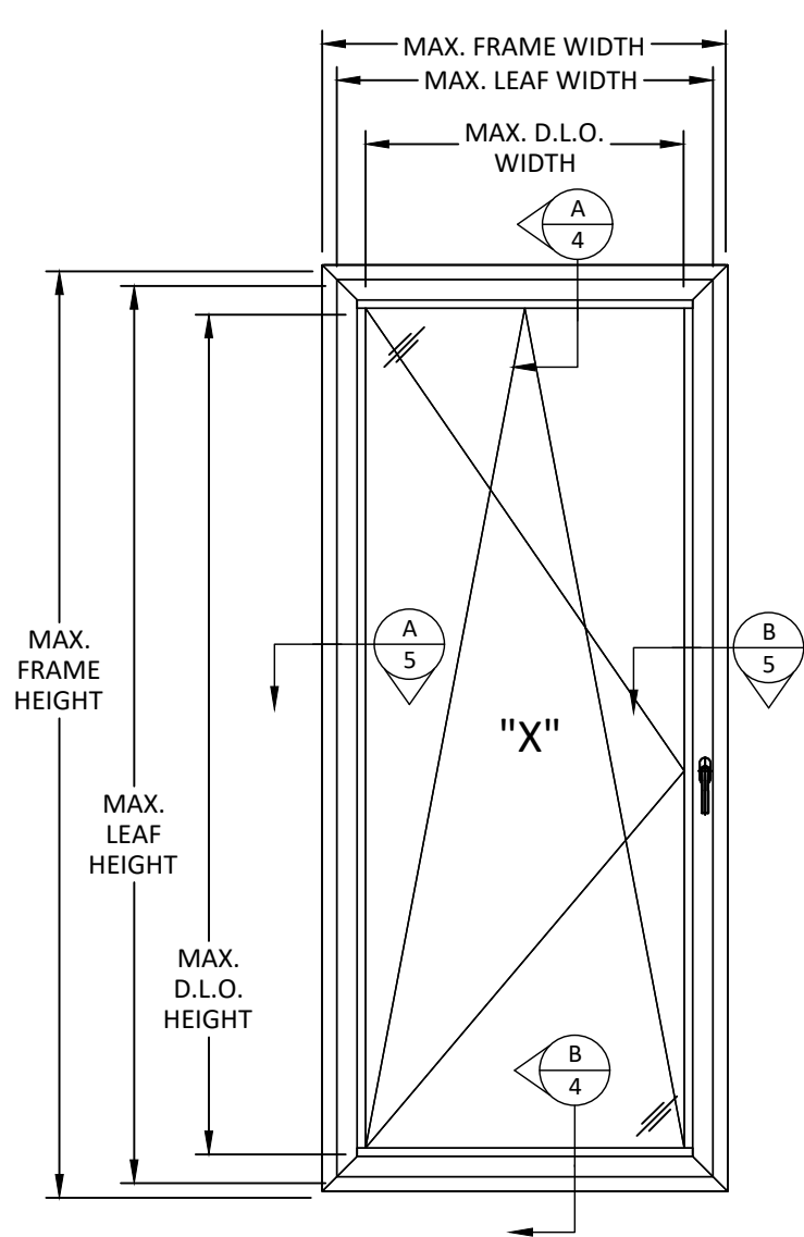
ELEVATIONS
